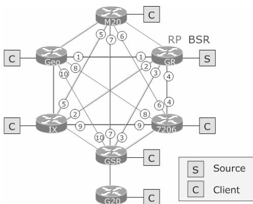
Fig. 5.5. Connection Topology of Basic Interoperability Evaluation
