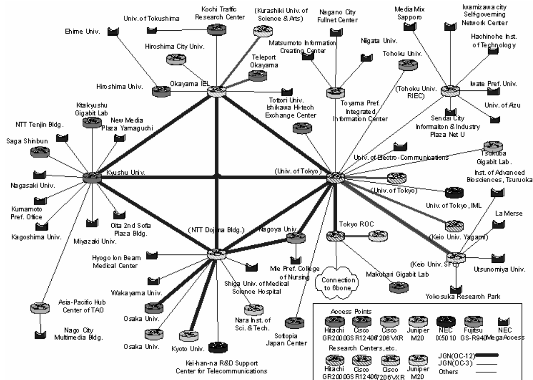
Fig. 2.1. JGN IPv6 Network Topology
