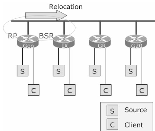
Fig. 5.8. BSR Function Verification
