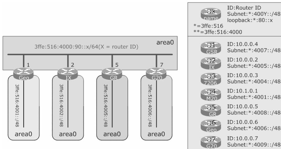
Fig. 5.3. Network Topology of the Evaluation in Ethernet Connection
