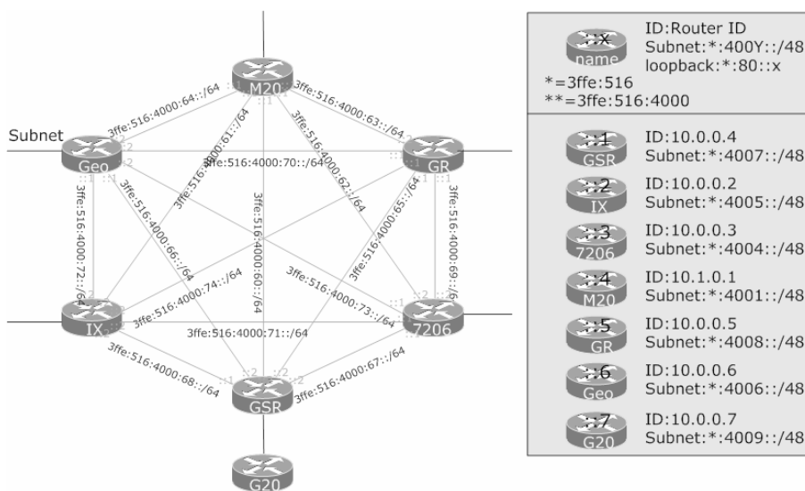
Fig. 5.2. Network Topology of the Evaluation in ATM Connection
