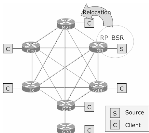
Fig. 5.7. Evaluation of RP Function
