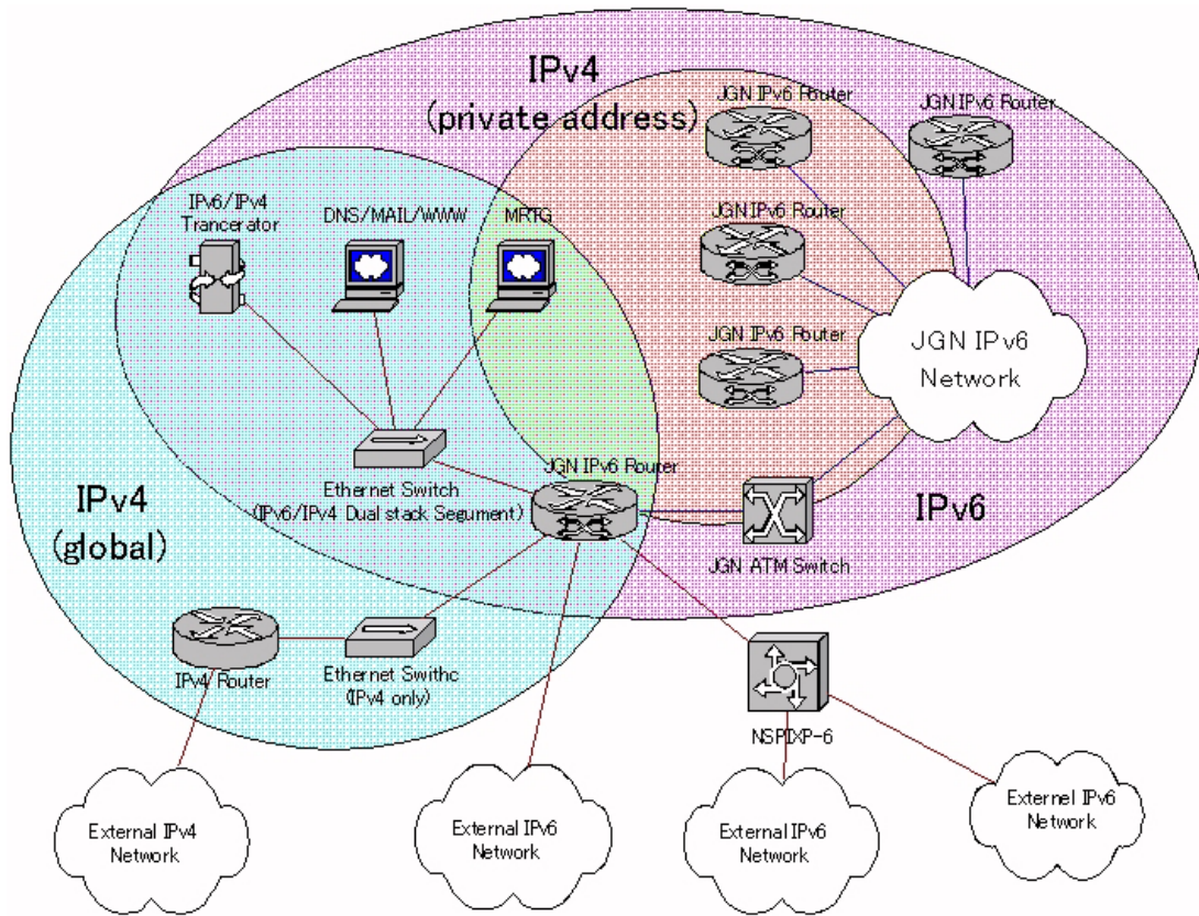
Fig. 3.6. IPv6 and IPv4 Operational Overview
