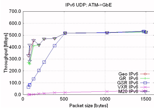
Fig. 4.2. Evaluation of Router's Throughput(II)
