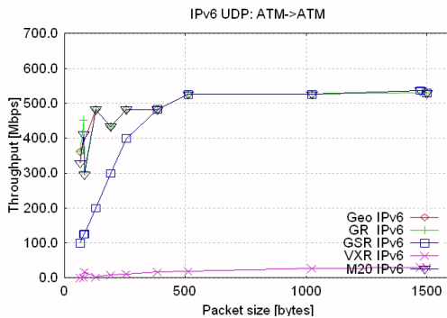
Fig. 4.1. Evaluation of Router's Throughput(I)
