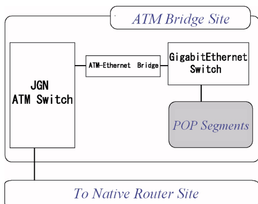
Fig. 3.5. Default configuration of bridge site
